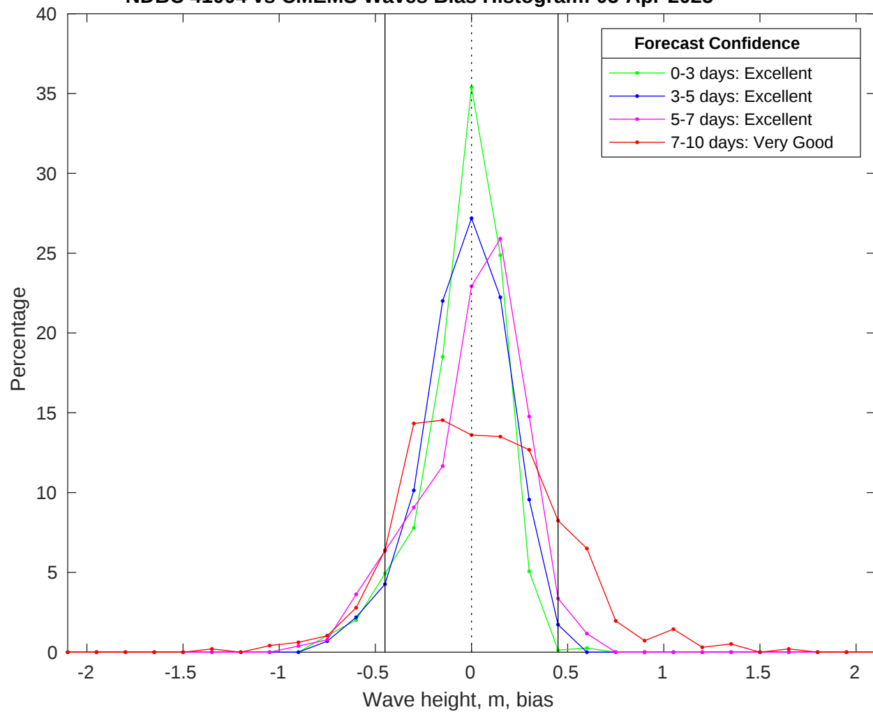
NDBC 41004 vs CMEMS Waves Bias Histogram: 05-Apr-2025
