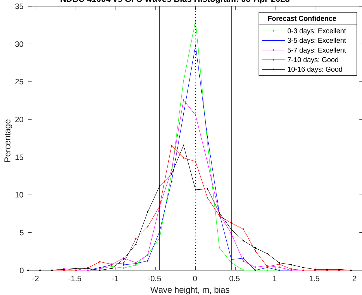
NDBC 41004 vs GFS Waves Bias Histogram: 05-Apr-2025
