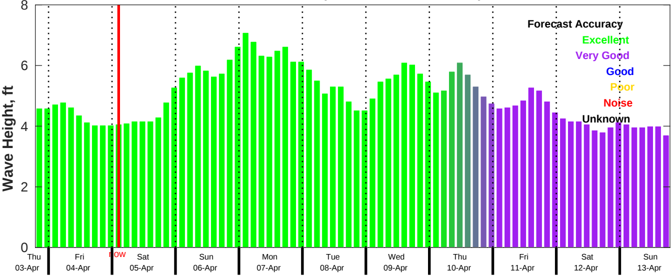
CMEMS Wave Forecast for NDBC 41004 from 03-Apr-2025 19:00:00 to 13-Apr-2025 19:00:00
