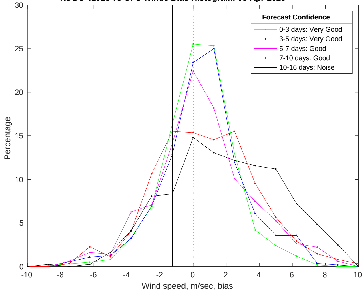
NDBC 41013 vs GFS Winds Bias Histogram: 05-Apr-2025
