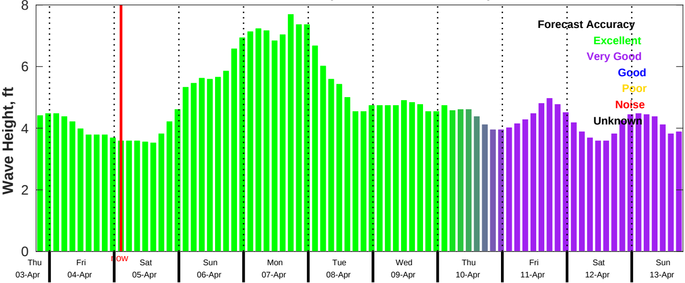
CMEMS Wave Forecast for NDBC 41013 from 03-Apr-2025 19:00:00 to 13-Apr-2025 19:00:00
