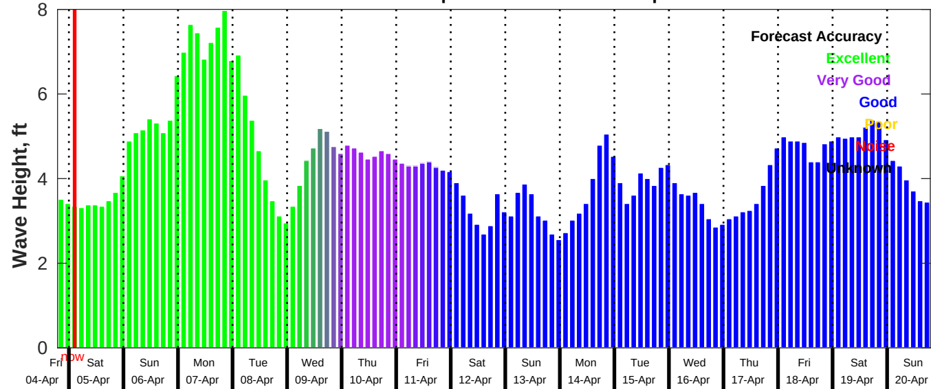
GFS Wave Forecast for NDBC 41013 from 04-Apr-2025 19:00:00 to 20-Apr-2025 19:00:00
