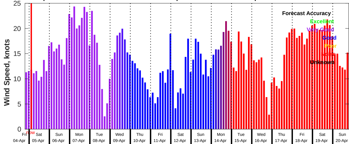
GFS Wind Speed Forecast for NDBC 41013 from 04-Apr-2025 19:00:00 to 20-Apr-2025 19:00:00
