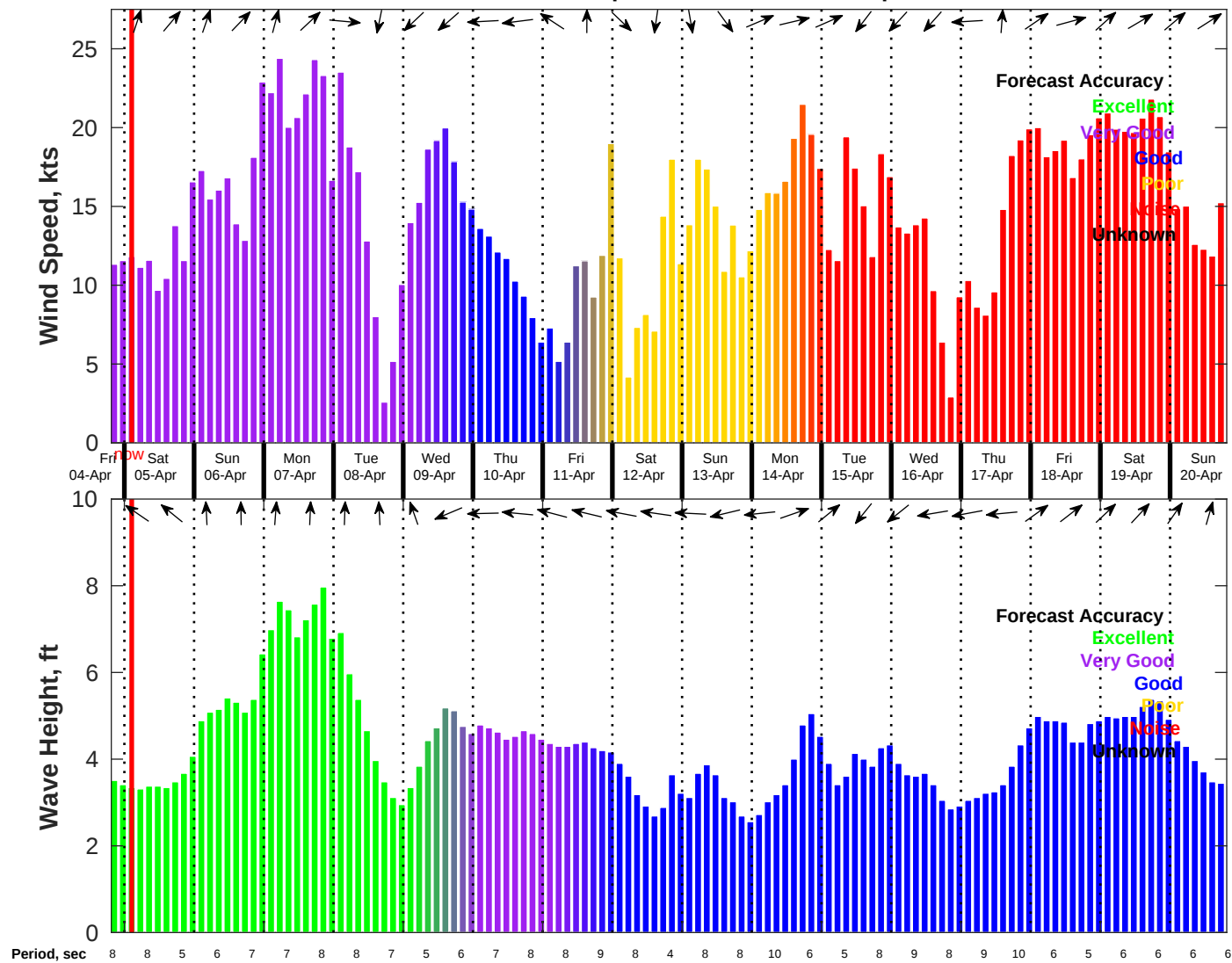
Wind & Wave Forecast for NDBC 41013 from 04-Apr-2025 19:00:00 to 20-Apr-2025 19:00:00
