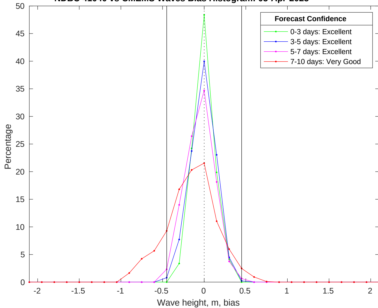
NDBC 41040 vs CMEMS Waves Bias Histogram: 05-Apr-2025
