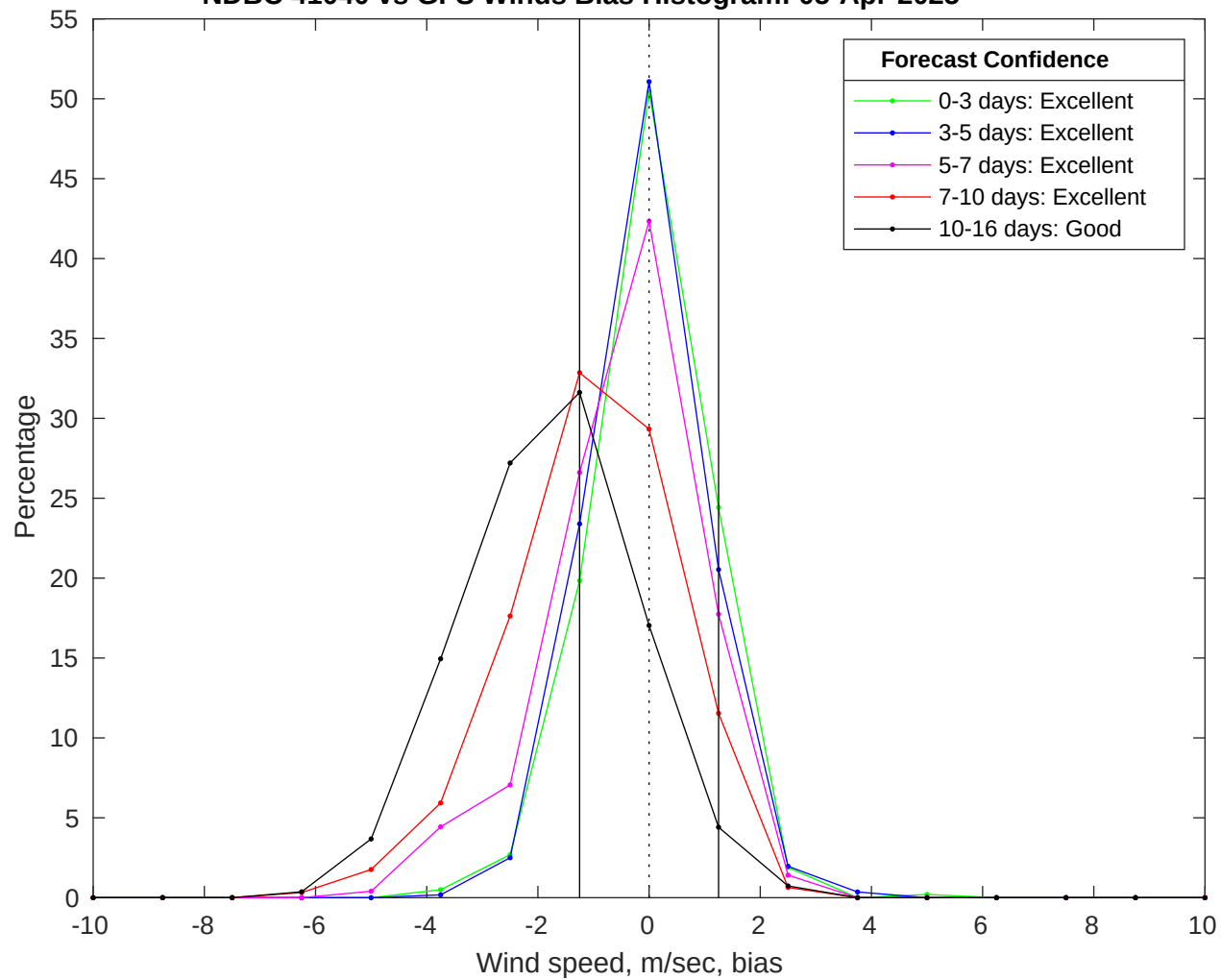
NDBC 41040 vs GFS Winds Bias Histogram: 05-Apr-2025
