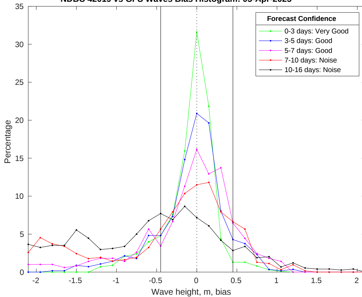
NDBC 42019 vs GFS Waves Bias Histogram: 05-Apr-2025
