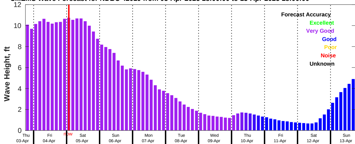
CMEMS Wave Forecast for NDBC 42019 from 03-Apr-2025 18:00:00 to 13-Apr-2025 18:00:00
