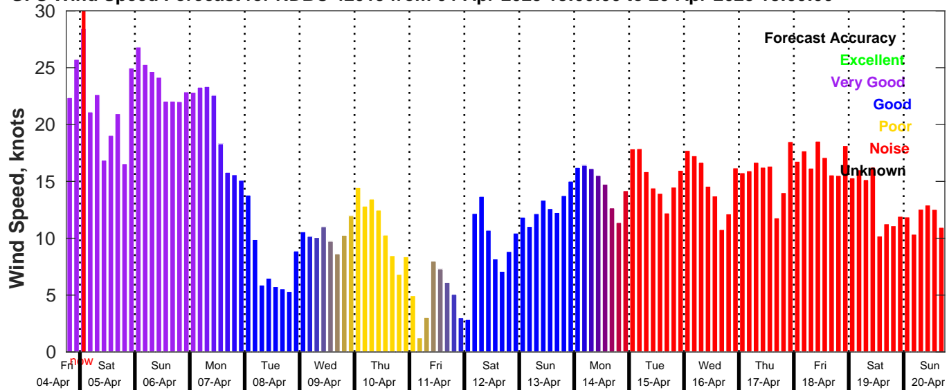
GFS Wind Speed Forecast for NDBC 42019 from 04-Apr-2025 18:00:00 to 20-Apr-2025 18:00:00
