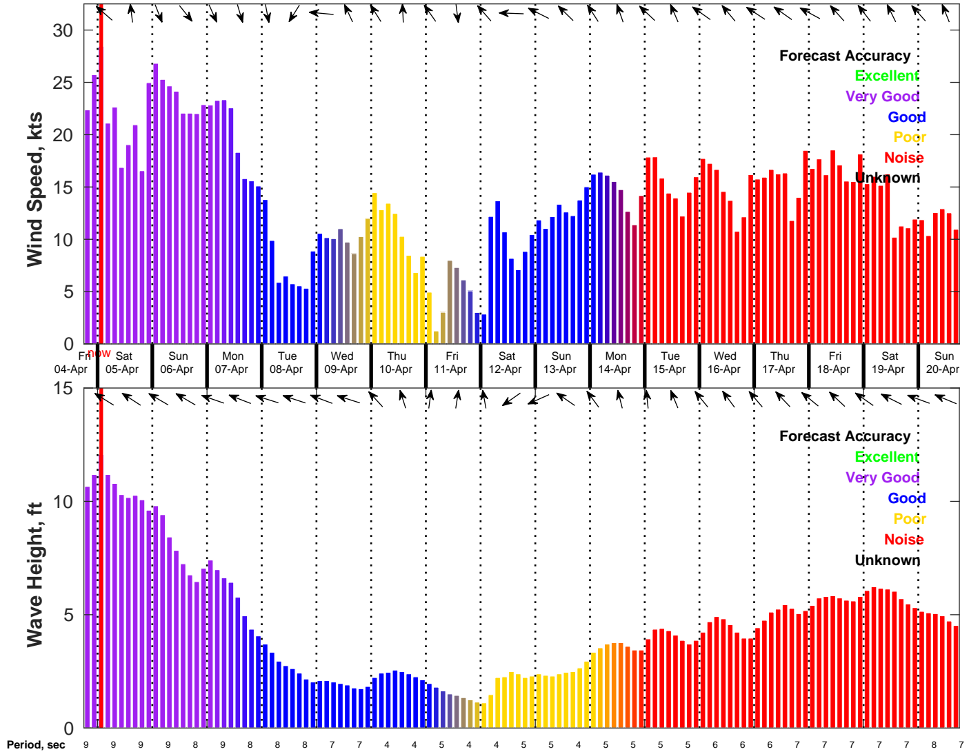
Wind & Wave Forecast for NDBC 42019 from 04-Apr-2025 18:00:00 to 20-Apr-2025 18:00:00
