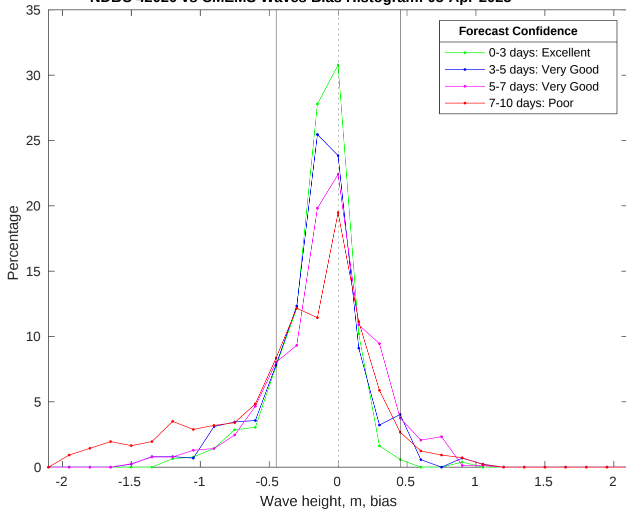
NDBC 42020 vs CMEMS Waves Bias Histogram: 05-Apr-2025
