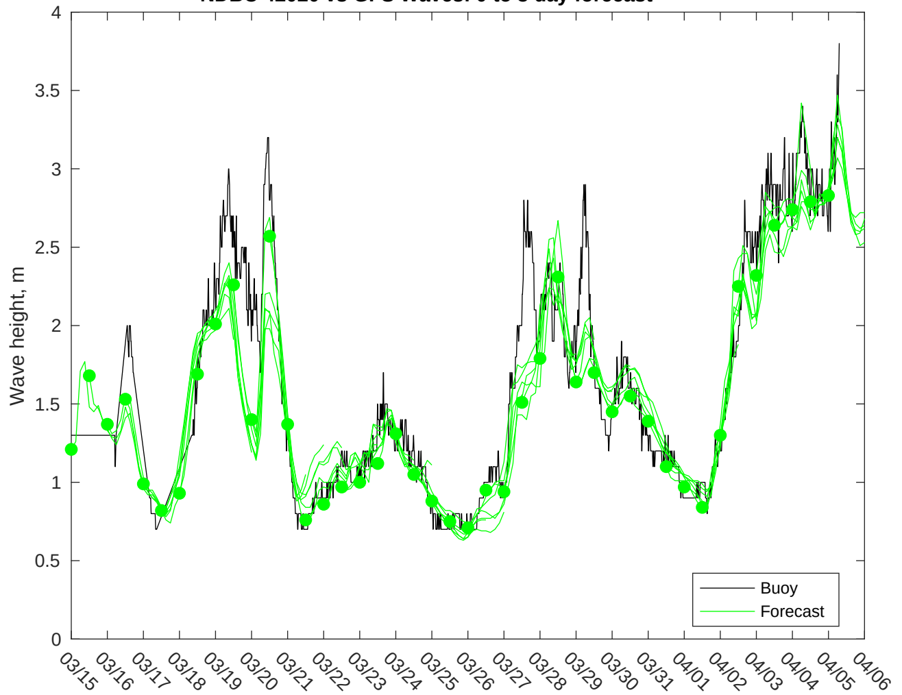
NDBC 42020 vs GFS Waves: 0 to 3 day forecast
