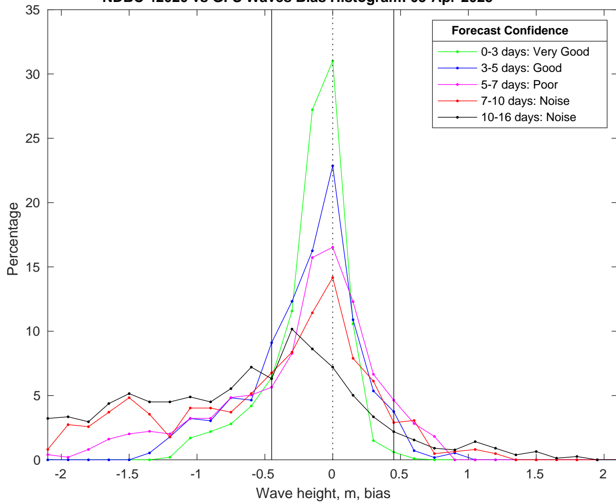
NDBC 42020 vs GFS Waves Bias Histogram: 05-Apr-2025
