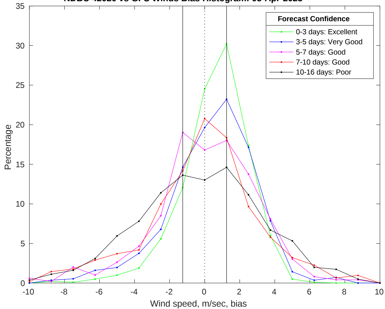
NDBC 42020 vs GFS Winds Bias Histogram: 05-Apr-2025
