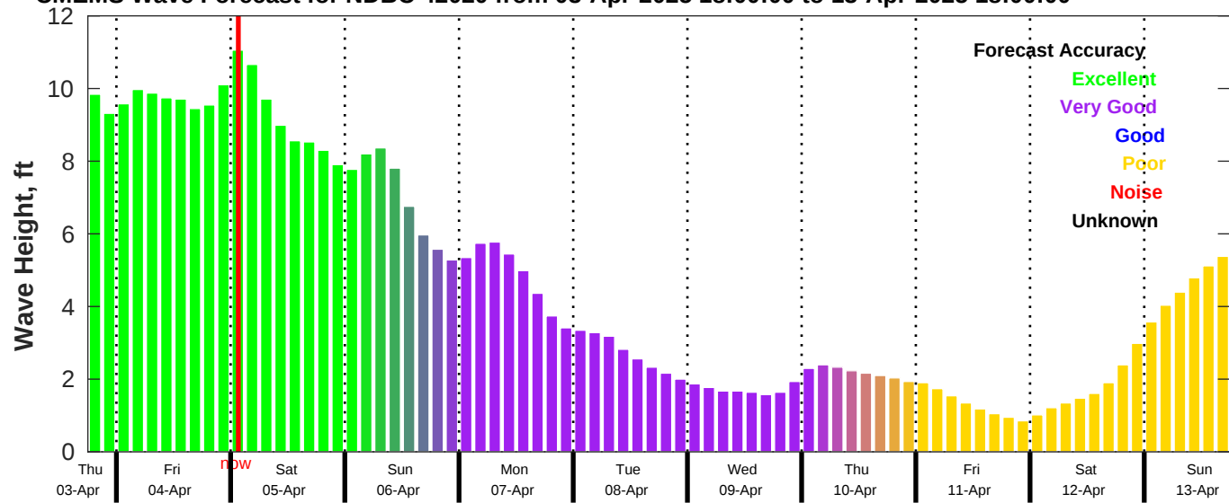
CMEMS Wave Forecast for NDBC 42020 from 03-Apr-2025 18:00:00 to 13-Apr-2025 18:00:00
