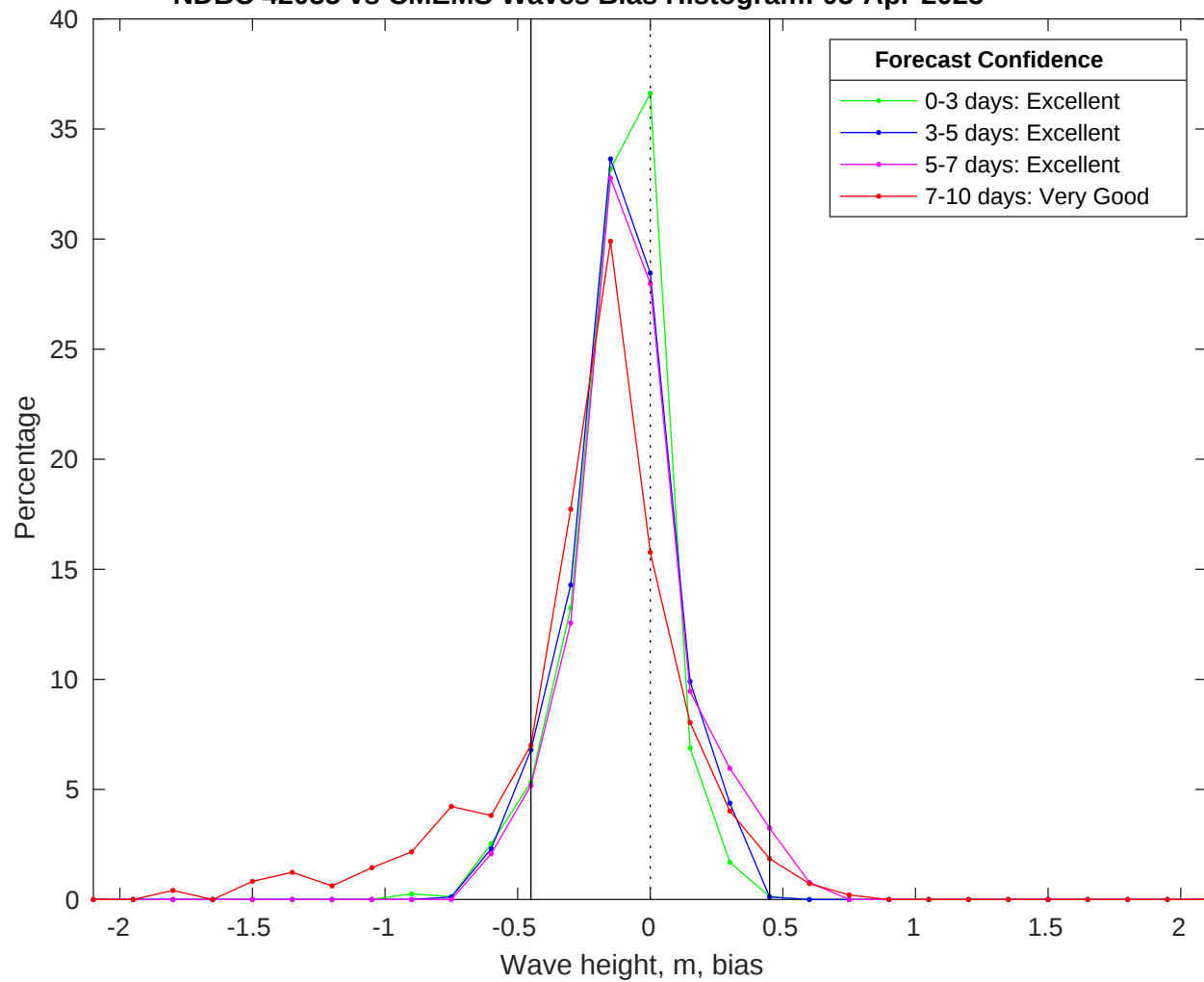
NDBC 42035 vs CMEMS Waves Bias Histogram: 05-Apr-2025
