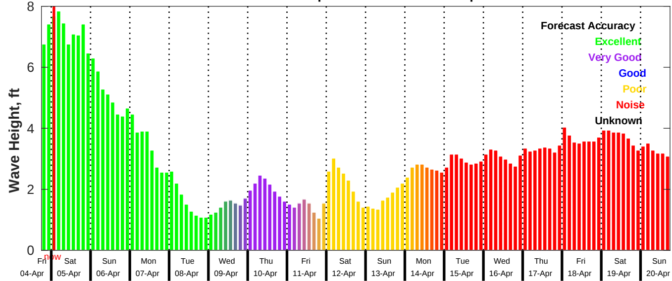
GFS Wave Forecast for NDBC 42035 from 04-Apr-2025 18:00:00 to 20-Apr-2025 18:00:00
