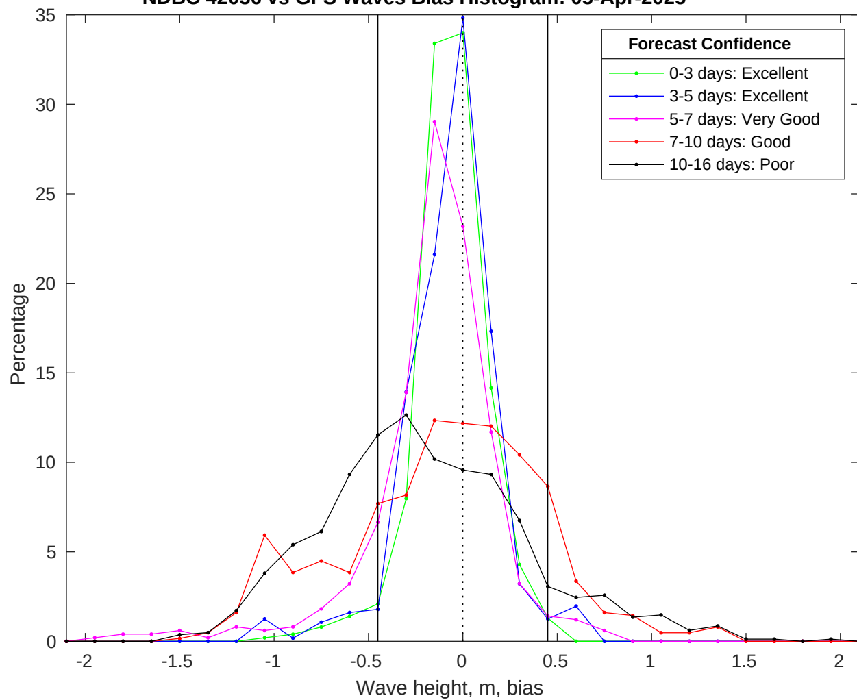
NDBC 42036 vs GFS Waves Bias Histogram: 05-Apr-2025
