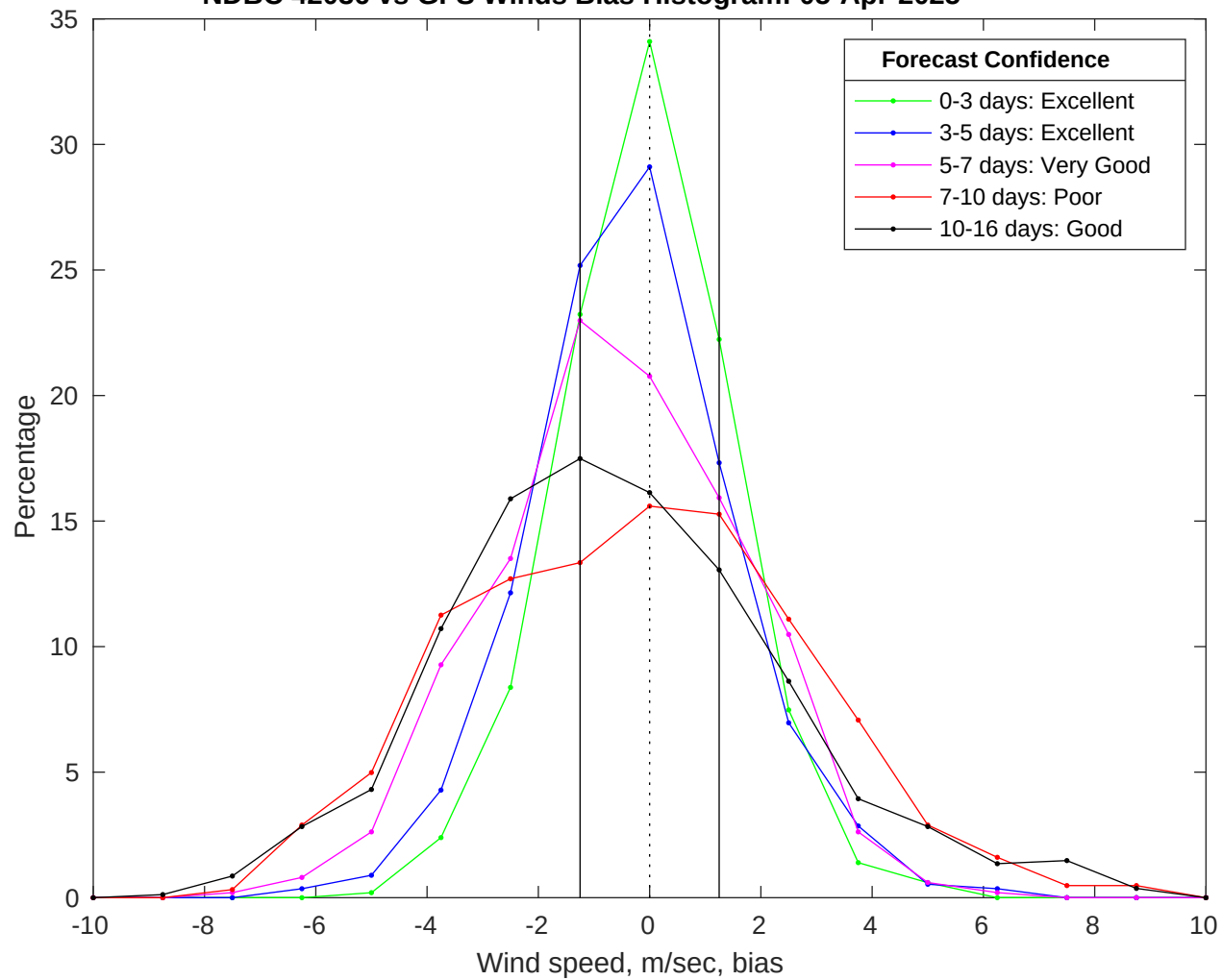
NDBC 42036 vs GFS Winds Bias Histogram: 05-Apr-2025
