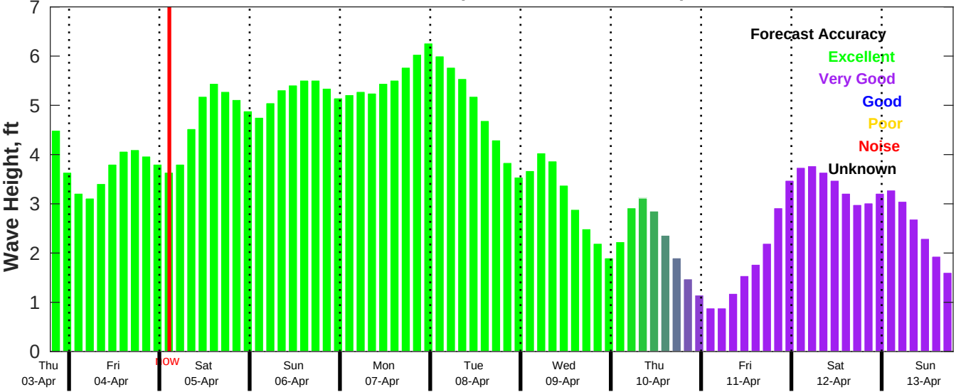
CMEMS Wave Forecast for NDBC 42036 from 03-Apr-2025 19:00:00 to 13-Apr-2025 19:00:00
