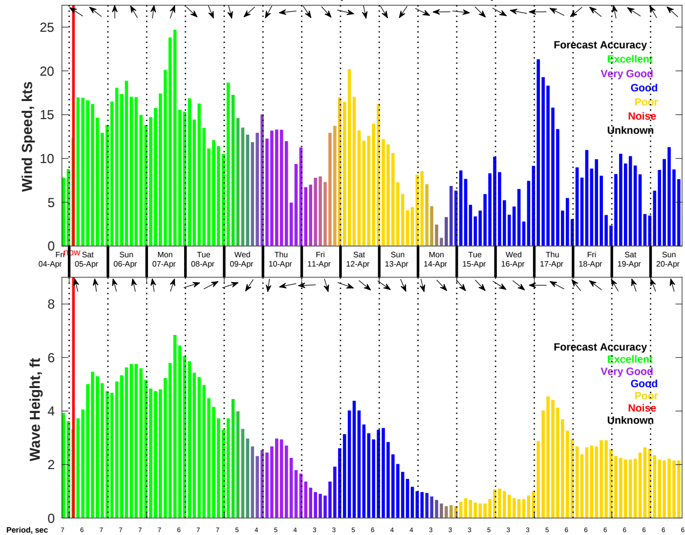
Wind & Wave Forecast for NDBC 42036 from 04-Apr-2025 19:00:00 to 20-Apr-2025 19:00:00
