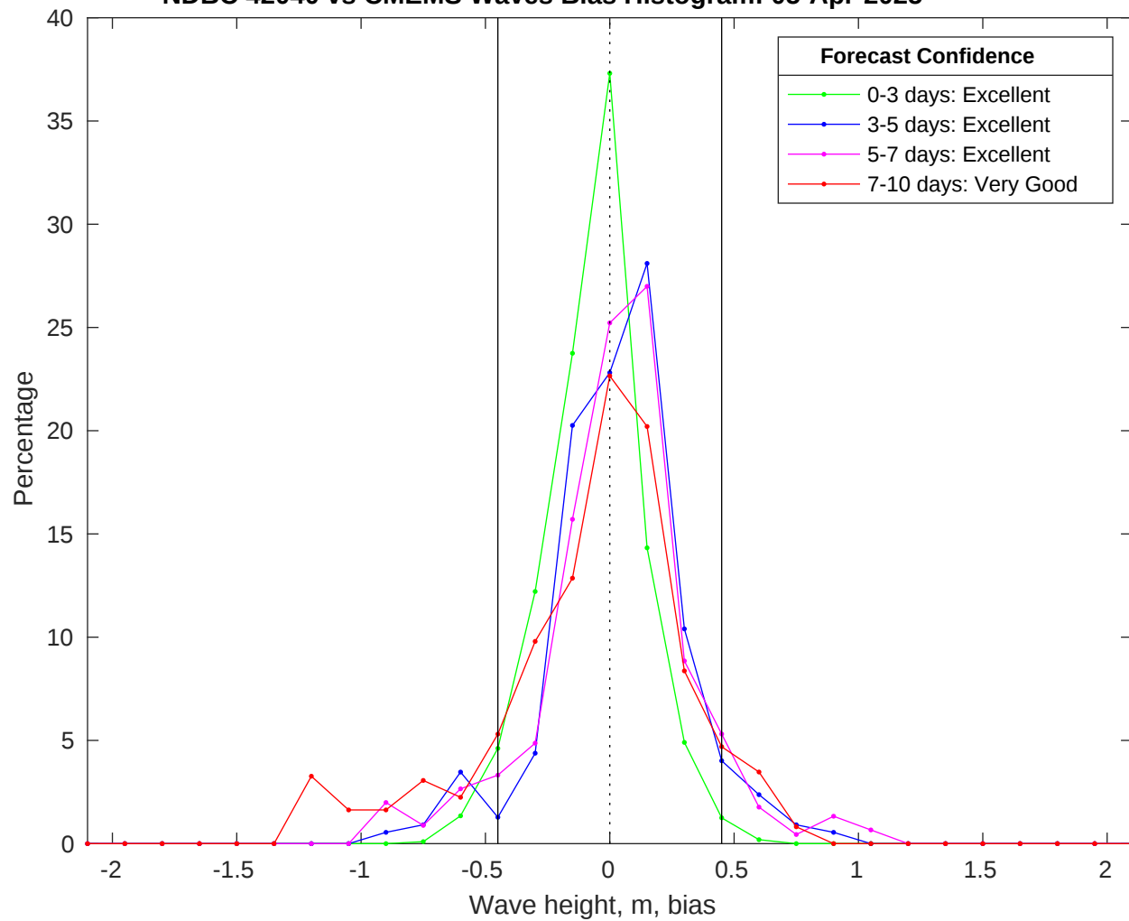
NDBC 42040 vs CMEMS Waves Bias Histogram: 05-Apr-2025
