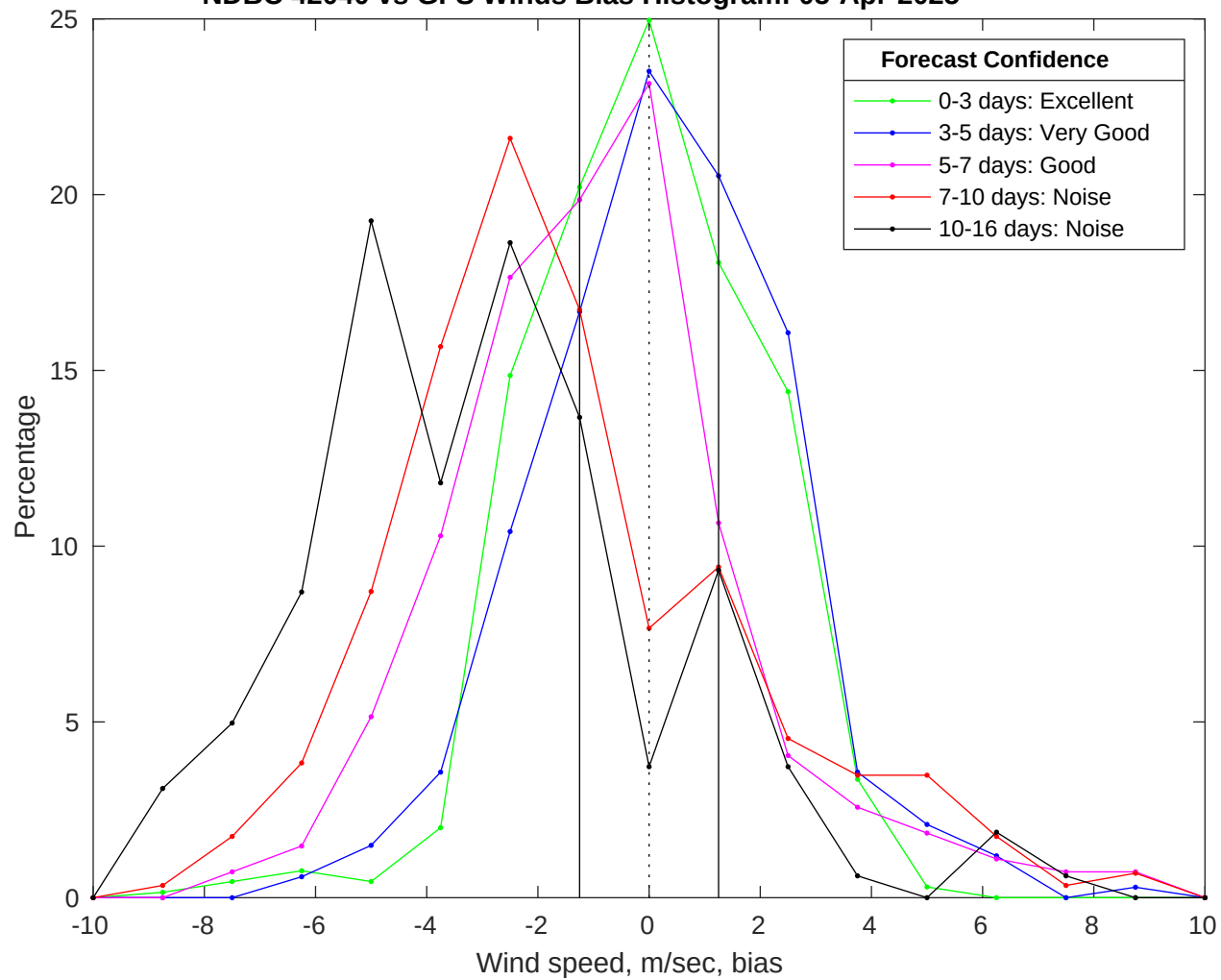
NDBC 42040 vs GFS Winds Bias Histogram: 05-Apr-2025
