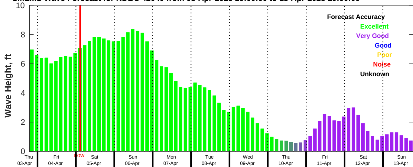
CMEMS Wave Forecast for NDBC 42040 from 03-Apr-2025 19:00:00 to 13-Apr-2025 19:00:00
