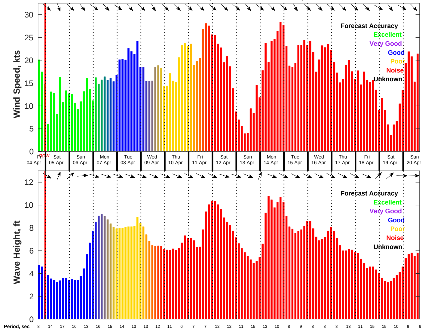
Wind & Wave Forecast for NDBC 46011 from 04-Apr-2025 16:00:00 to 20-Apr-2025 16:00:00
