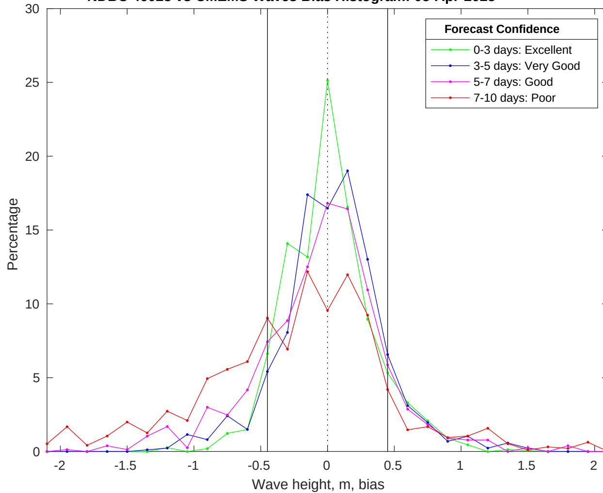
NDBC 46028 vs CMEMS Waves Bias Histogram: 05-Apr-2025
