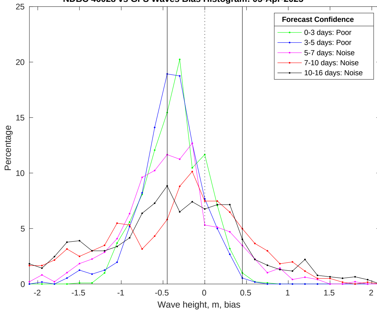
NDBC 46028 vs GFS Waves Bias Histogram: 05-Apr-2025
