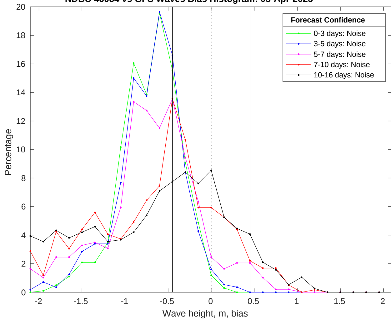
NDBC 46054 vs GFS Waves Bias Histogram: 05-Apr-2025
