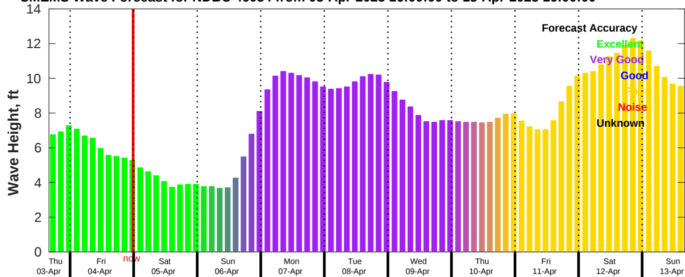
CMEMS Wave Forecast for NDBC 46054 from 03-Apr-2025 16:00:00 to 13-Apr-2025 16:00:00
