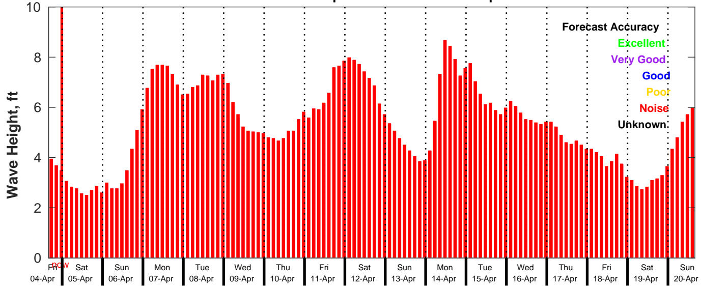
GFS Wave Forecast for NDBC 46054 from 04-Apr-2025 16:00:00 to 20-Apr-2025 16:00:00
