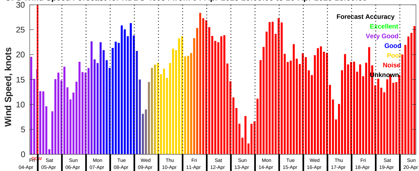
GFS Wind Speed Forecast for NDBC 46054 from 04-Apr-2025 16:00:00 to 20-Apr-2025 16:00:00
