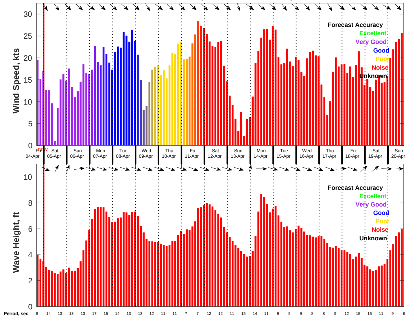
Wind & Wave Forecast for NDBC 46054 from 04-Apr-2025 16:00:00 to 20-Apr-2025 16:00:00
