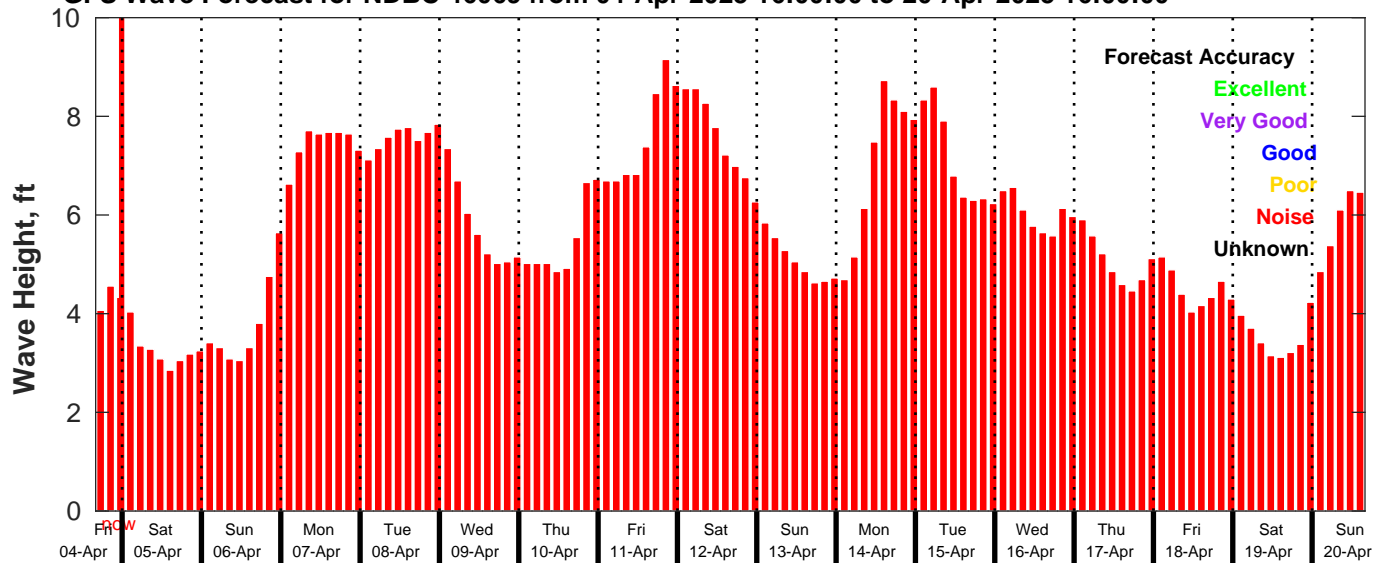
GFS Wave Forecast for NDBC 46069 from 04-Apr-2025 16:00:00 to 20-Apr-2025 16:00:00
