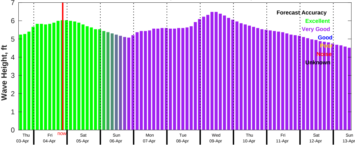
CMEMS Wave Forecast for NDBC 51209 from 03-Apr-2025 13:00:00 to 13-Apr-2025 13:00:00
