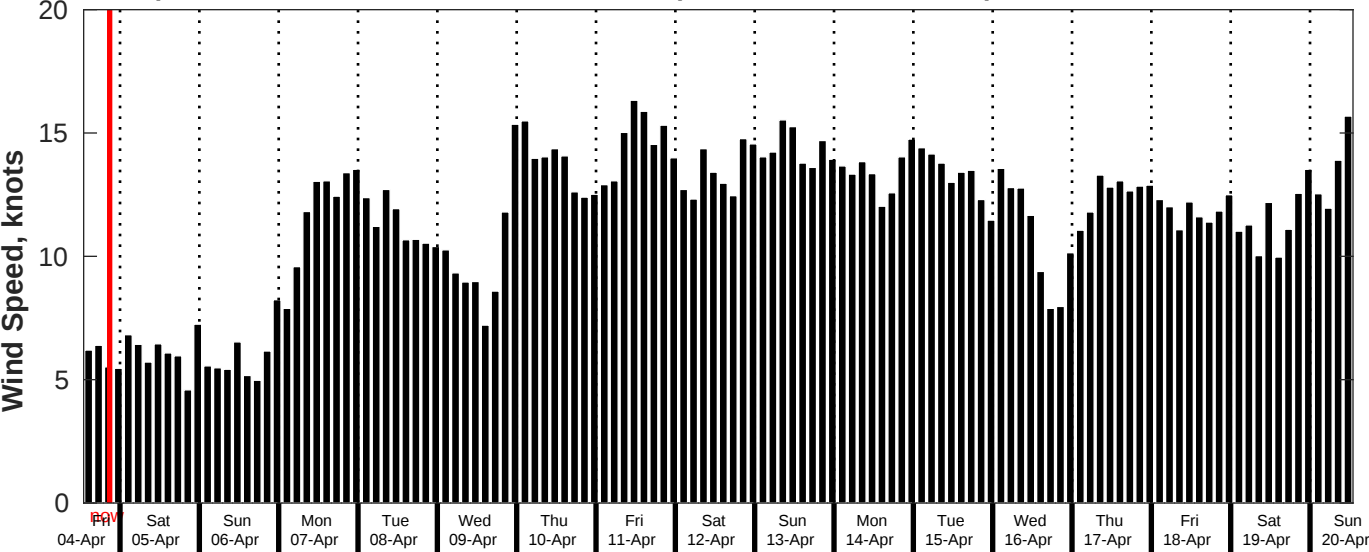
GFS Wind Speed Forecast for NDBC 51209 from 04-Apr-2025 13:00:00 to 20-Apr-2025 13:00:00
