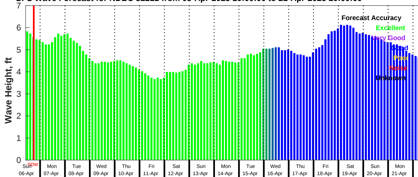
GFS Wave Forecast for NDBC 52211 from 05-Apr-2025 10:00:00 to 21-Apr-2025 10:00:00
