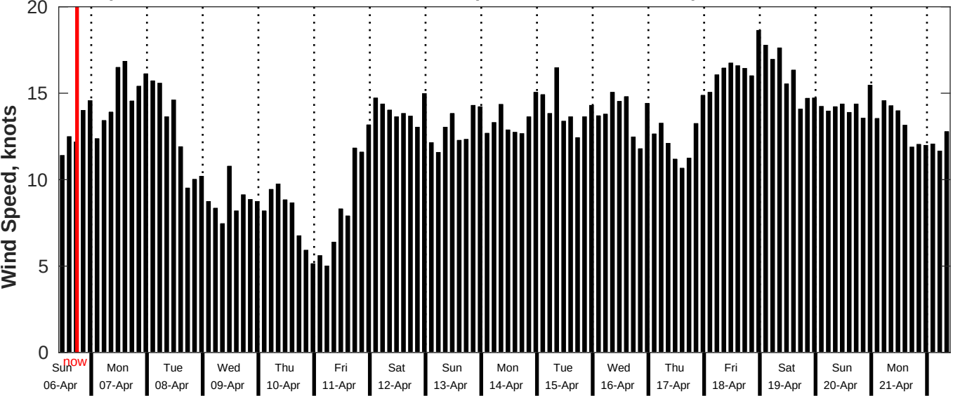
GFS Wind Speed Forecast for NDBC 52211 from 05-Apr-2025 10:00:00 to 21-Apr-2025 10:00:00
