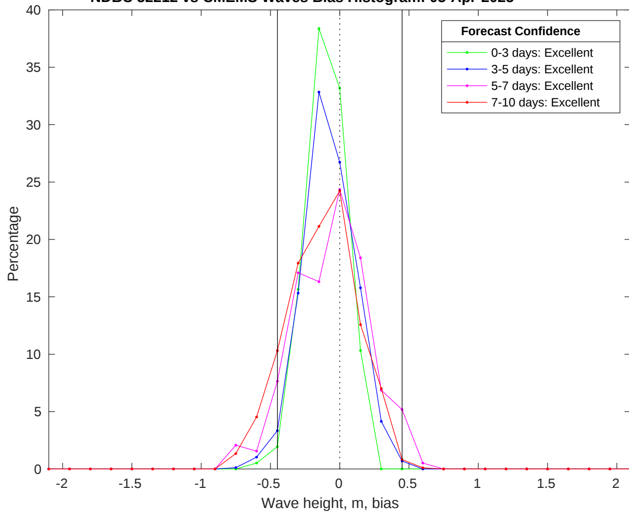
NDBC 52212 vs CMEMS Waves Bias Histogram: 05-Apr-2025
