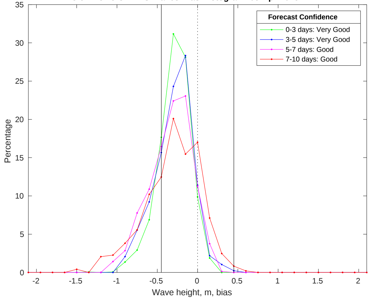
NDBC 52213 vs CMEMS Waves Bias Histogram: 05-Apr-2025
