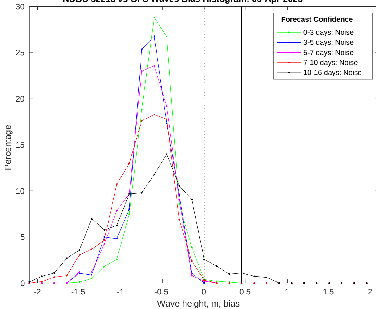
NDBC 52213 vs GFS Waves Bias Histogram: 05-Apr-2025
