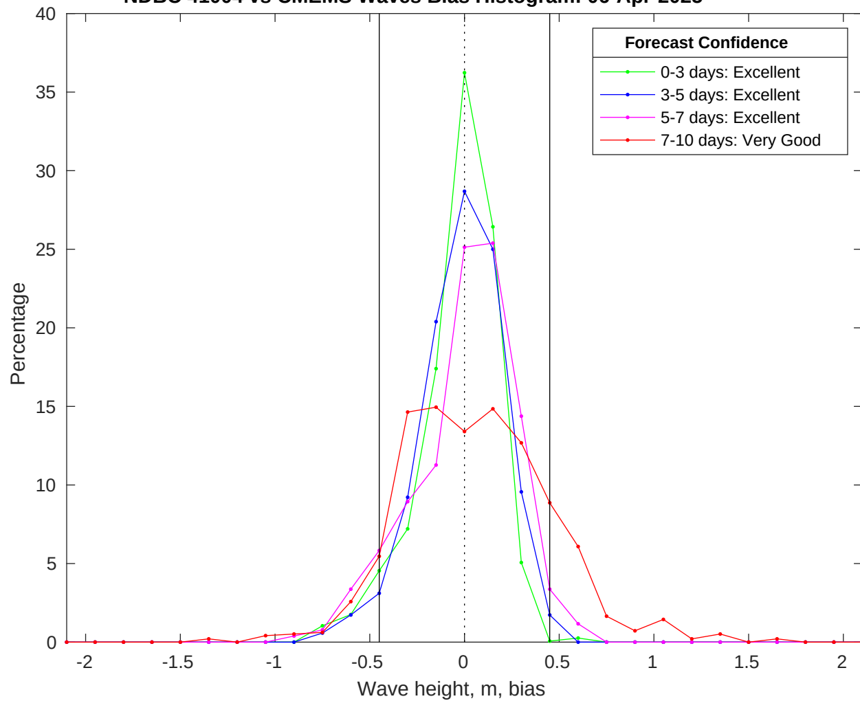
NDBC 41004 vs CMEMS Waves Bias Histogram: 06-Apr-2025
