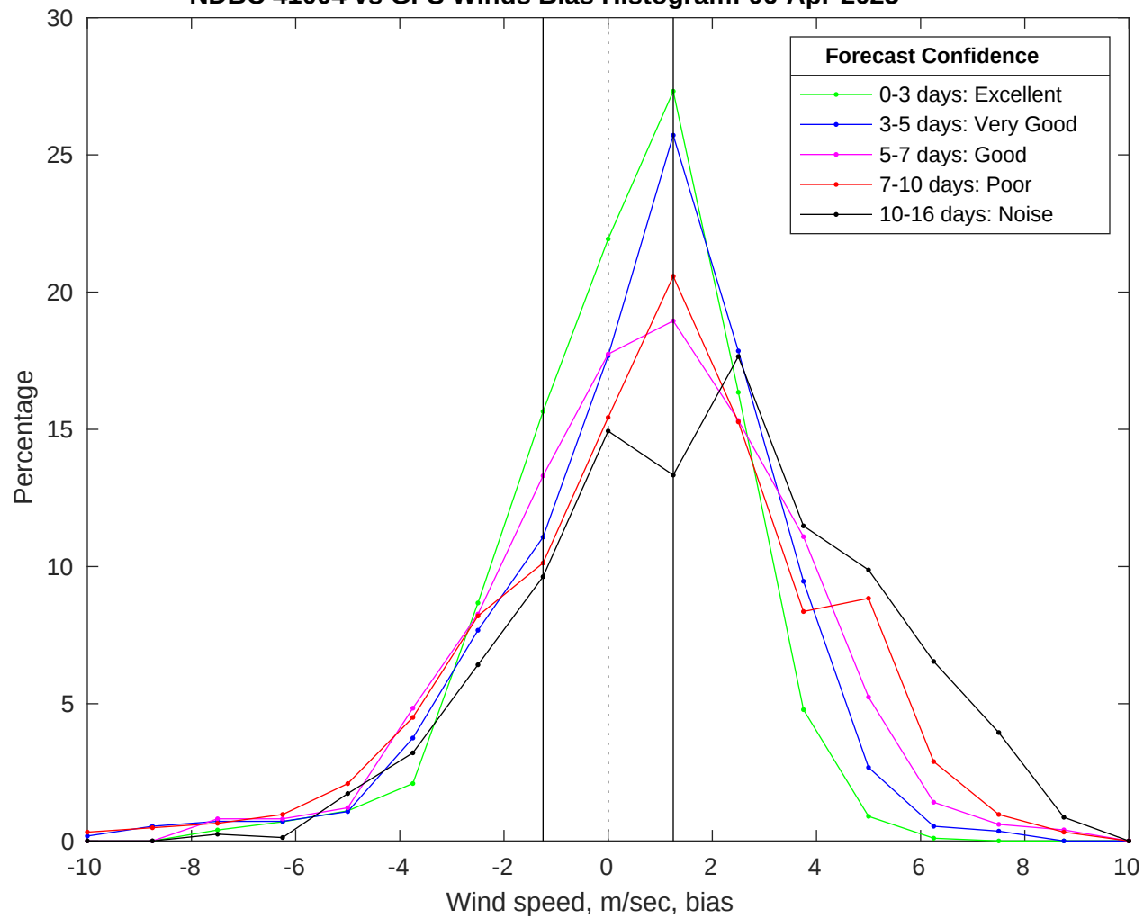
NDBC 41004 vs GFS Winds Bias Histogram: 06-Apr-2025
