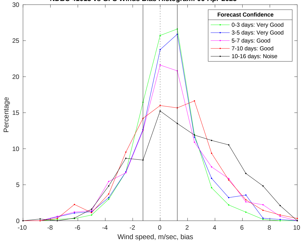
NDBC 41013 vs GFS Winds Bias Histogram: 06-Apr-2025
