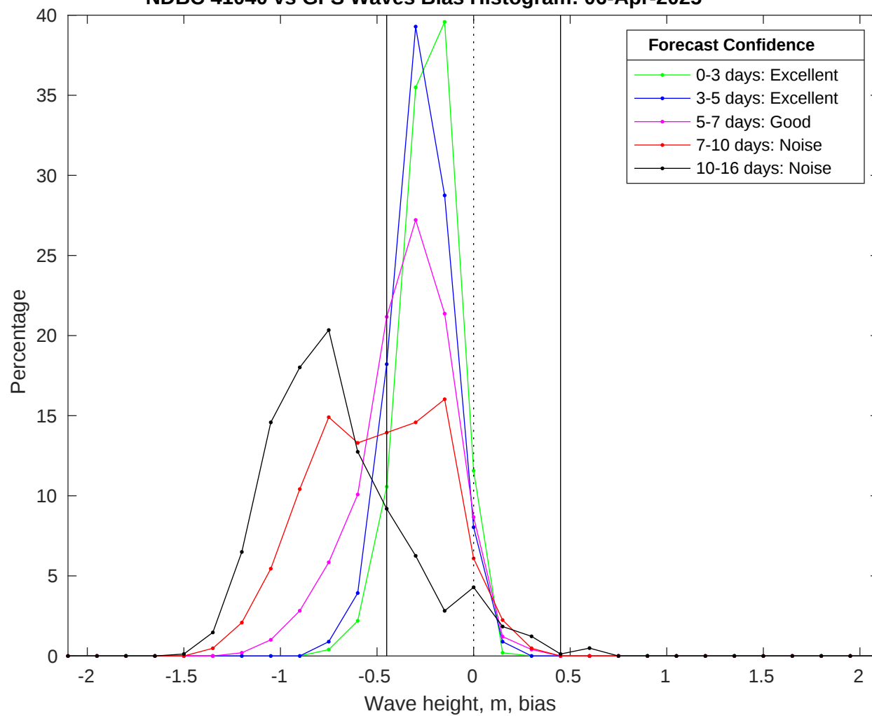
NDBC 41040 vs GFS Waves Bias Histogram: 06-Apr-2025
