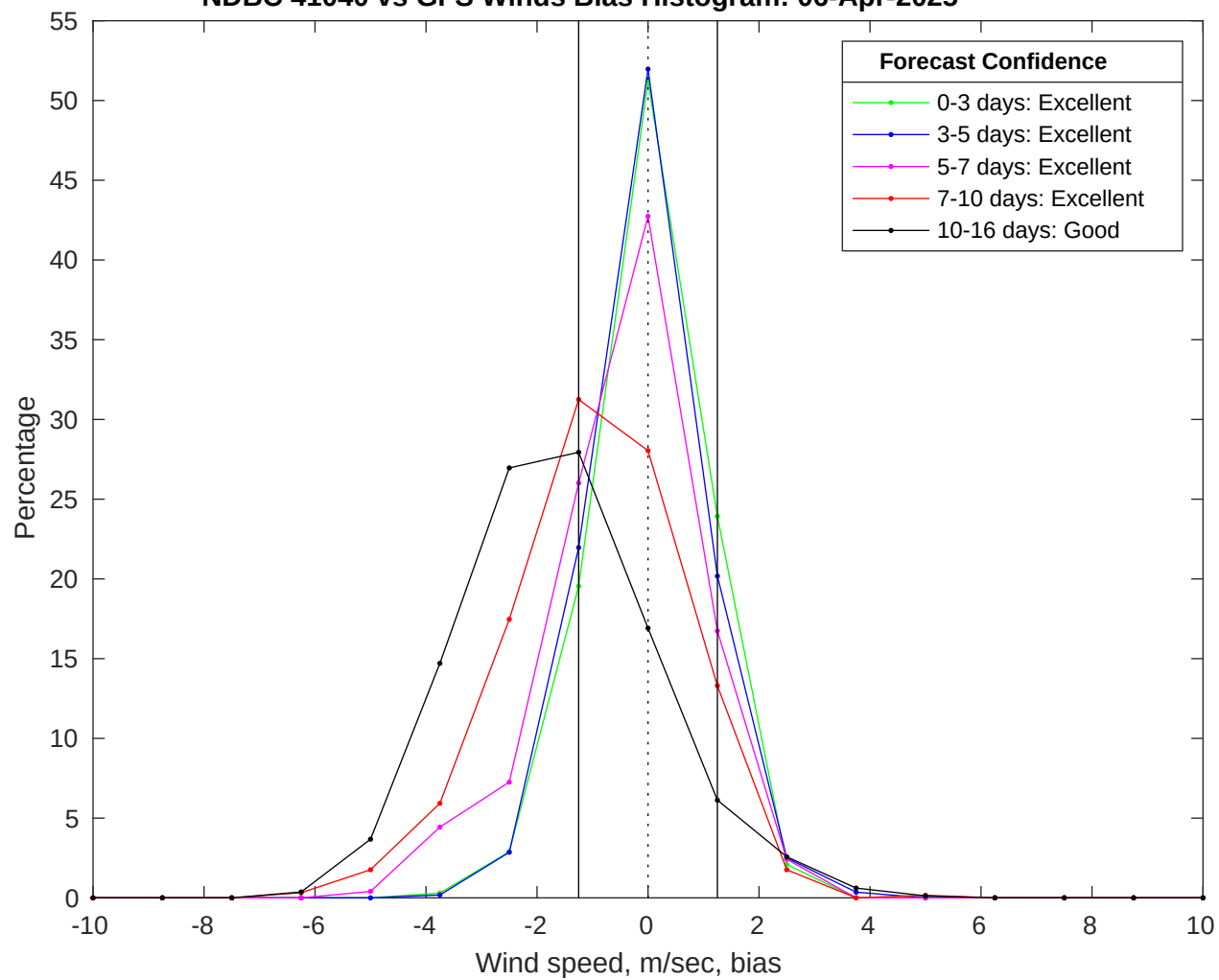
NDBC 41040 vs GFS Winds Bias Histogram: 06-Apr-2025
