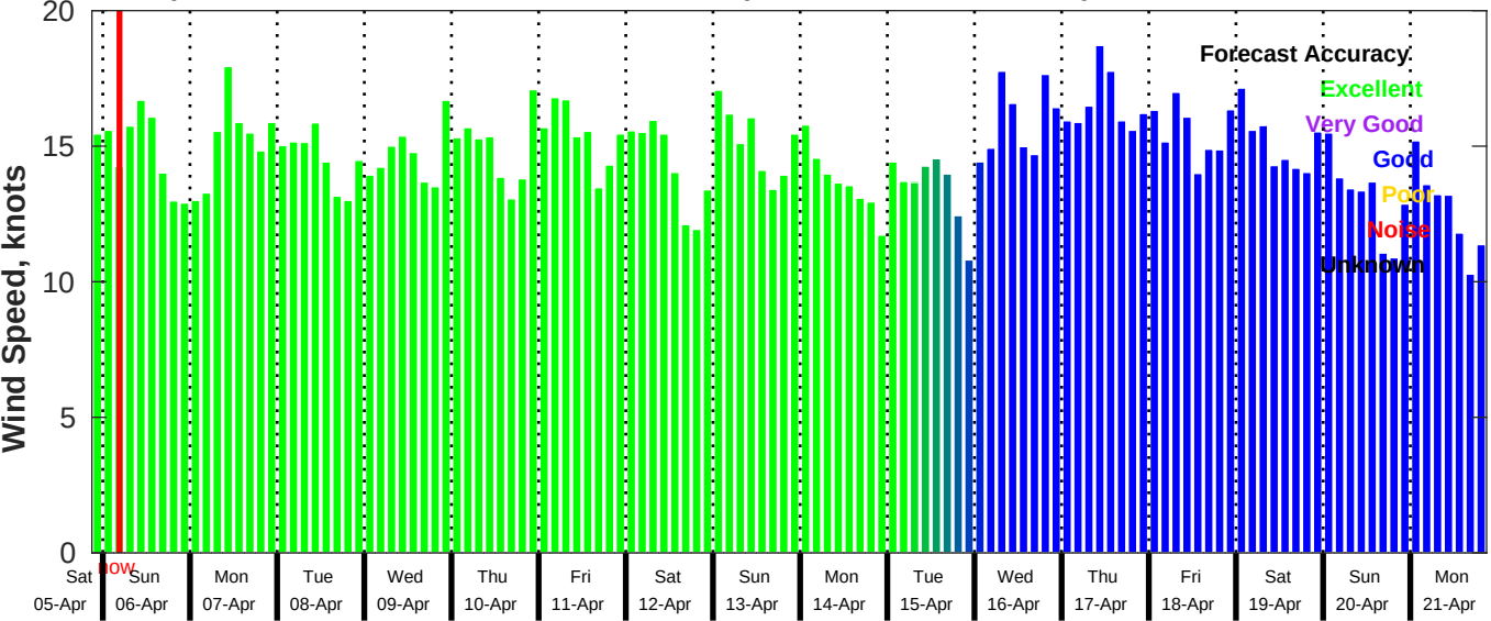
GFS Wind Speed Forecast for NDBC 41040 from 05-Apr-2025 21:00:00 to 21-Apr-2025 21:00:00
